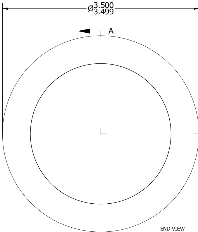
END VIEW SCALE 1 : 1
