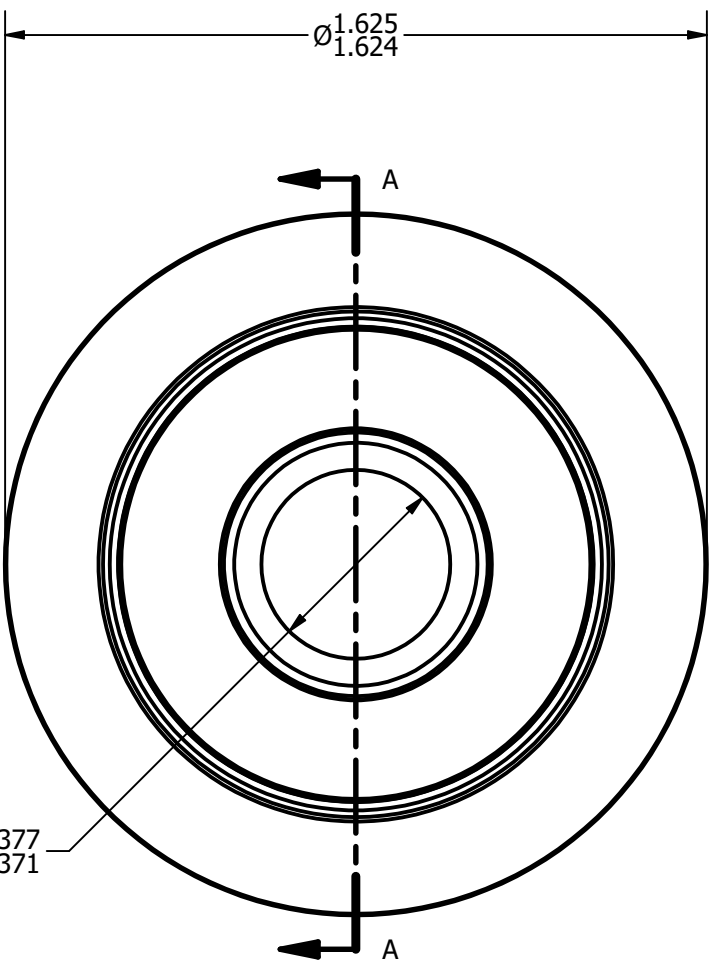
BASE VIEW SCALE 2.25 : 1
