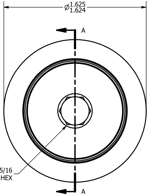
BASE VIEW SCALE 1.875 : 1
