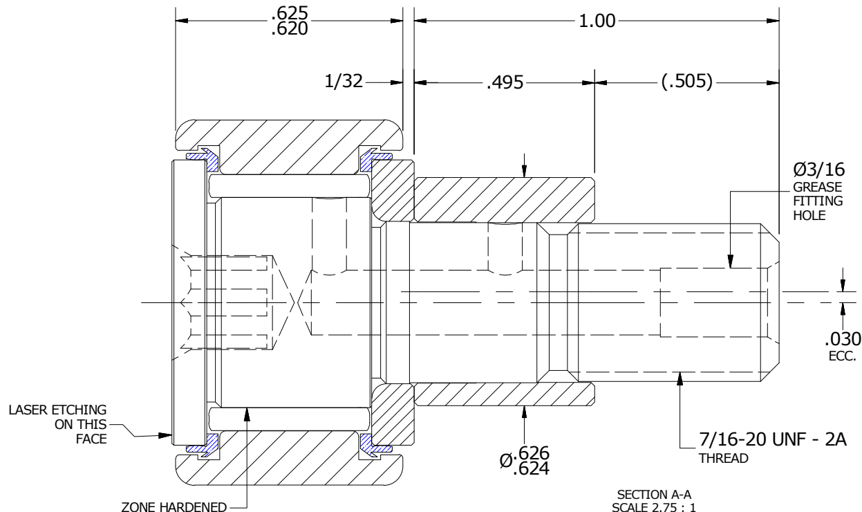
END VIEW SCALE 2.75 : 1
