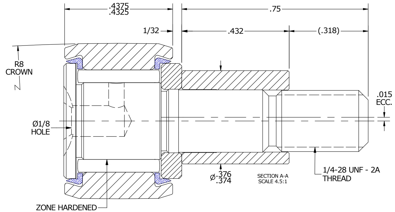
END VIEW SCALE 4.5:1
