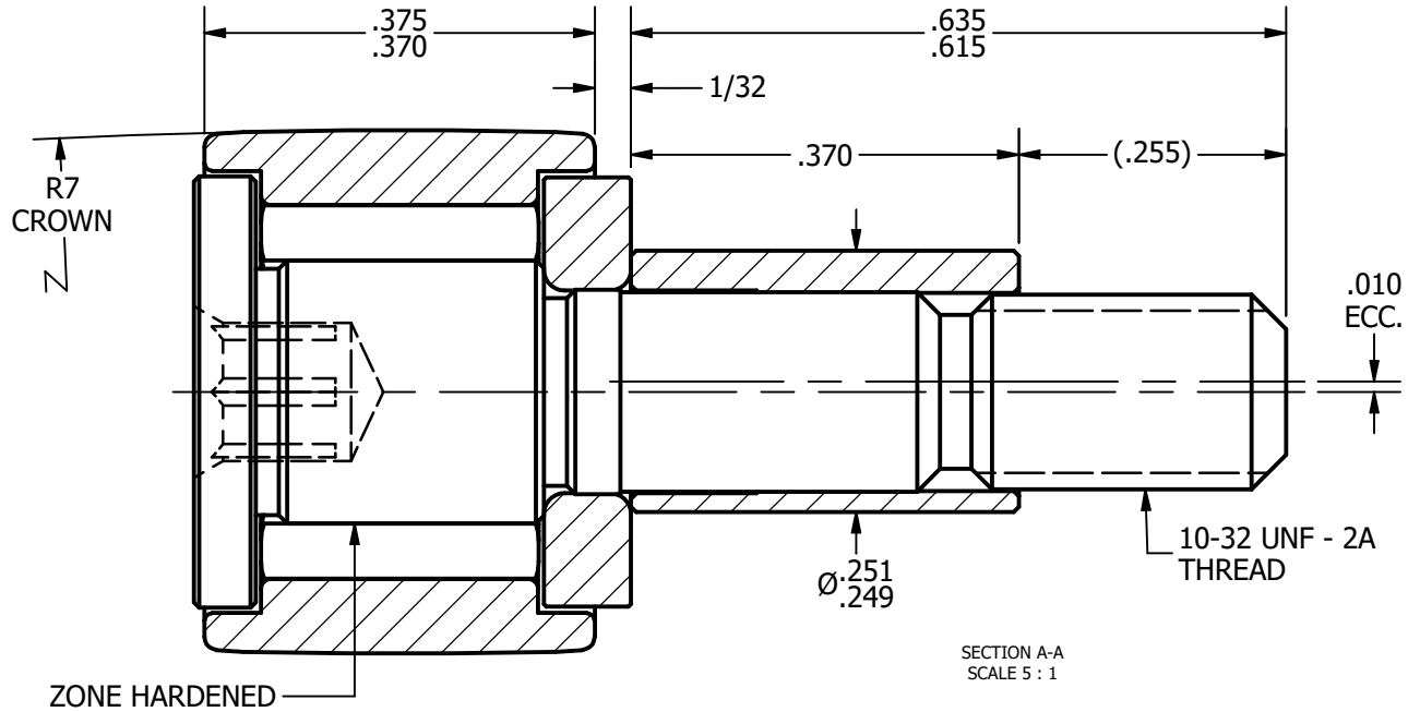
BASE VIEW SCALE 5 : 1
